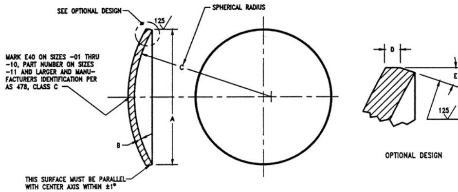
FIGURE 1 - PLUG
