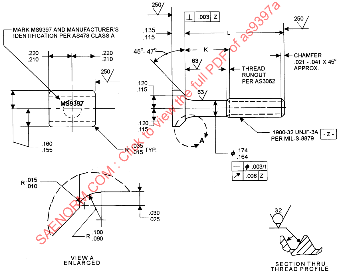
FIGURE 1 - BOLT
