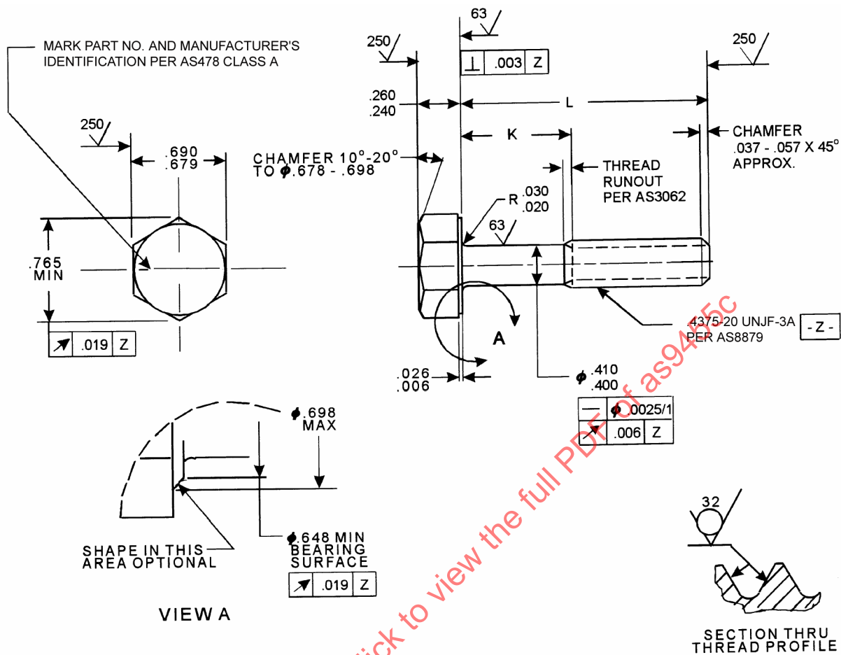
FIGURE 1 - BOLT
