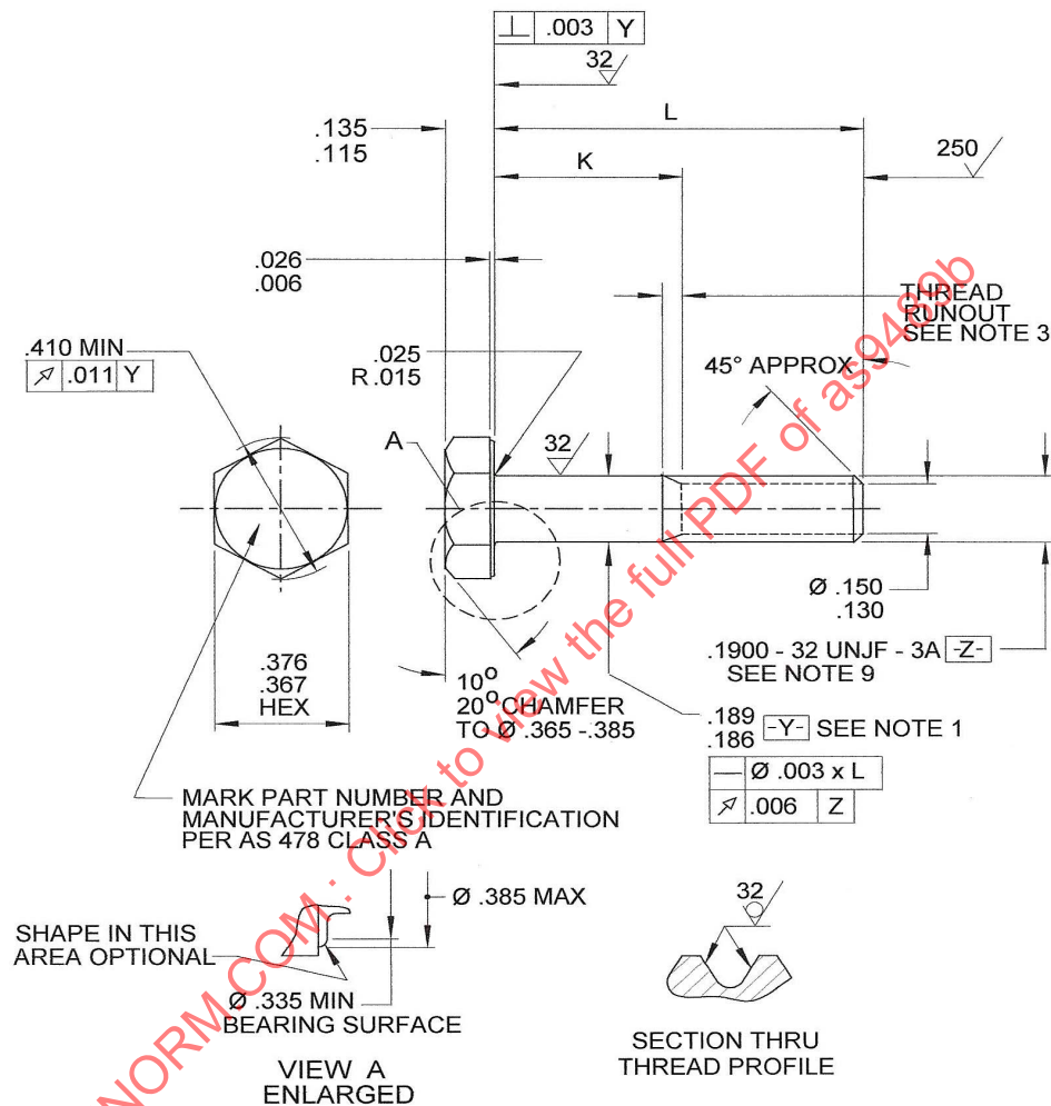
FIGURE 1 - BOLT
