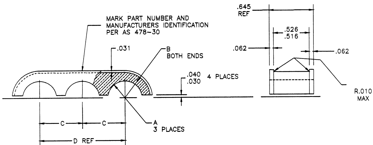
FIGURE 1. CLAMP LOOP CUSHION
