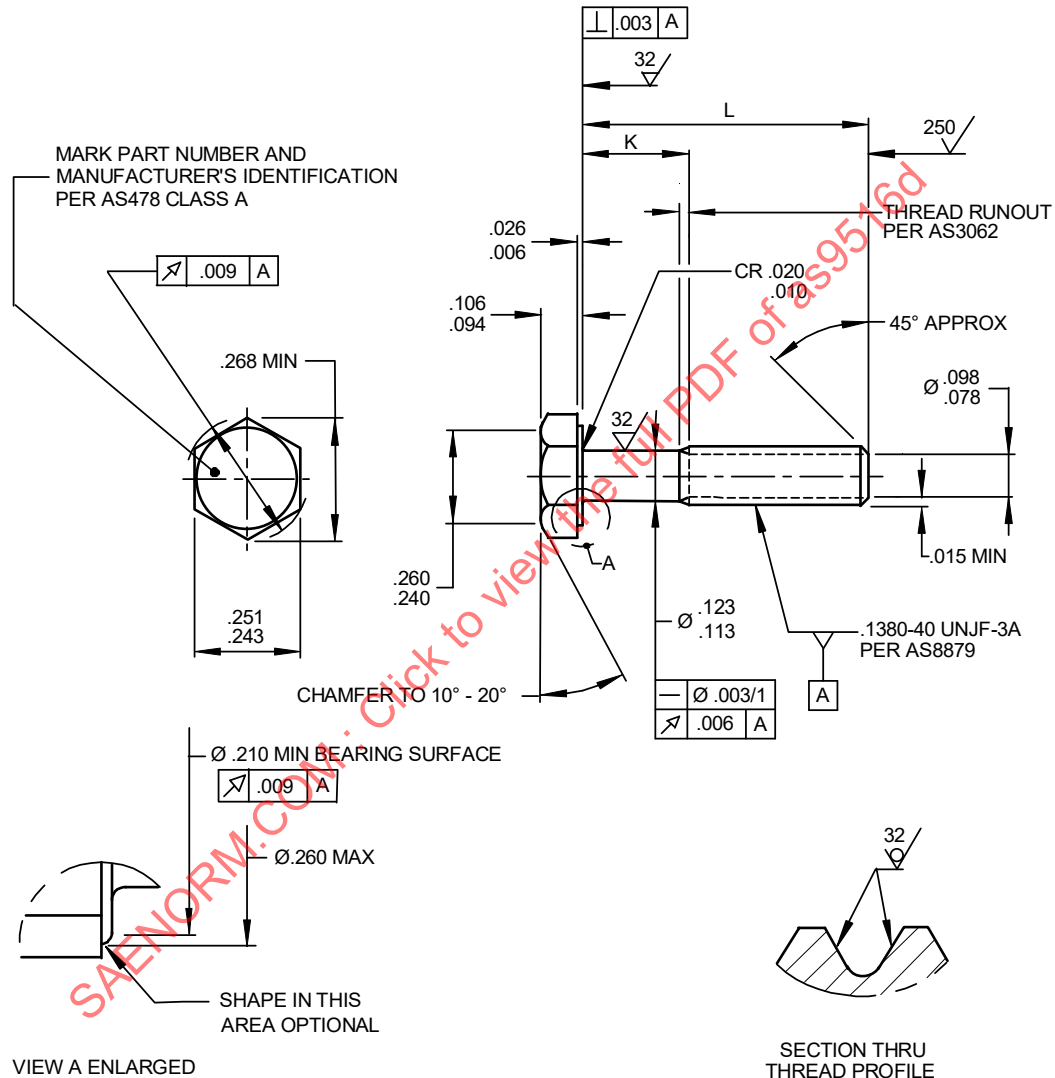
FIGURE 1 - SCREW
