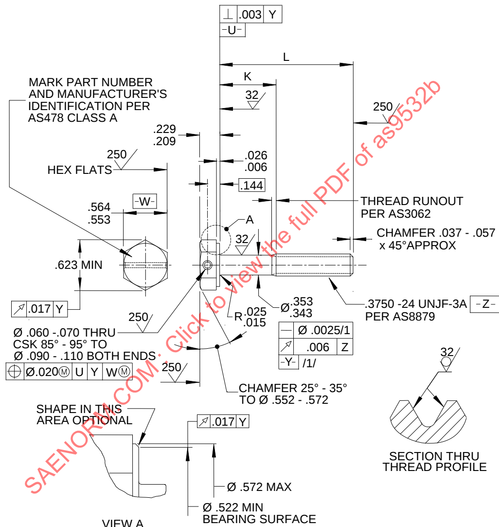
FIGURE 1 - BOLT
