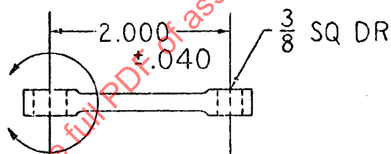
TORQUE ADAPTER
