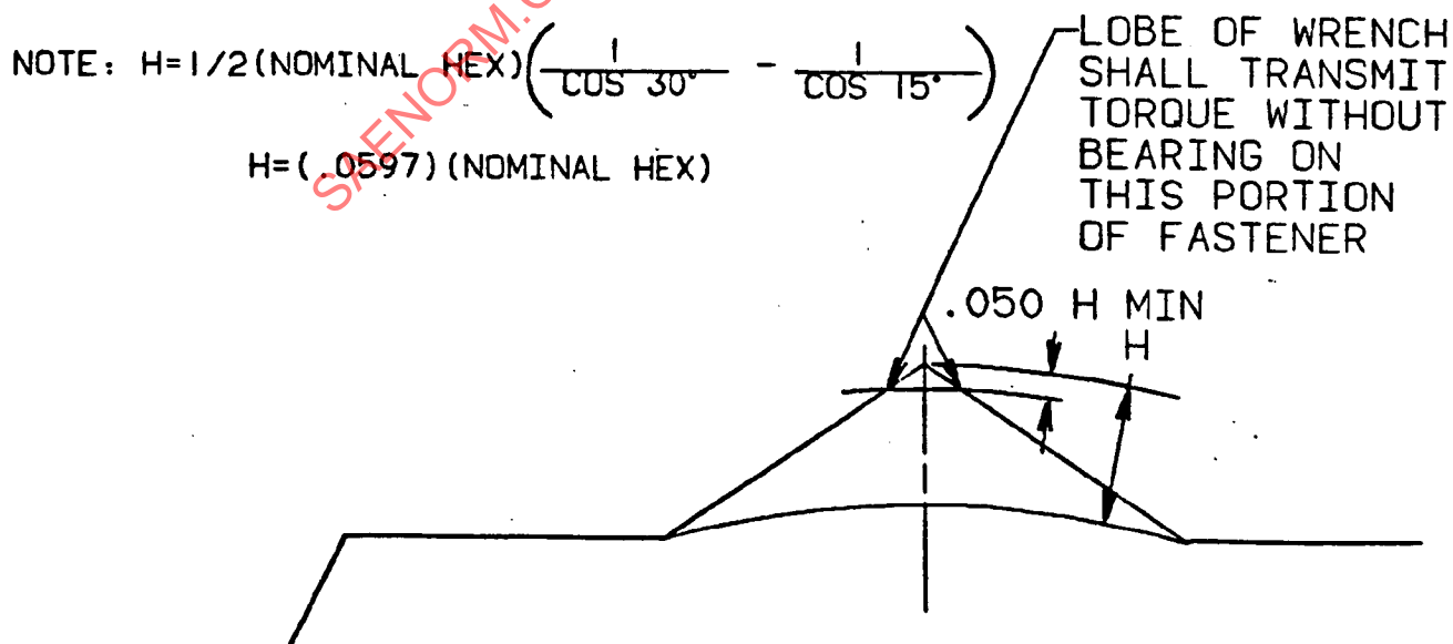
FIGURE 1 - Internal Wrench Engagement
