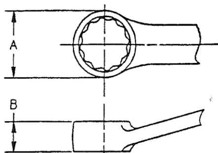
FIGURE 9 - TYPE II BOX WRENCH
