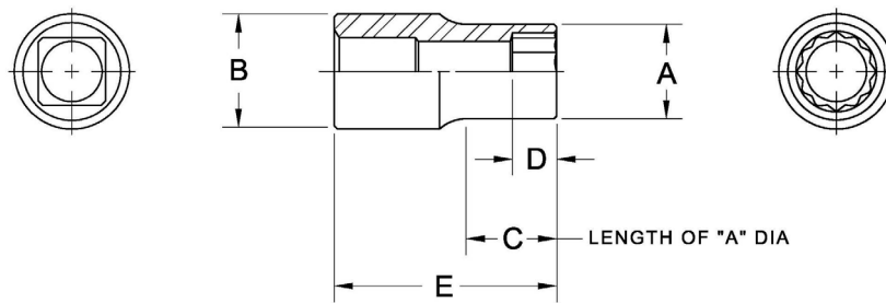
FIGURE 3 - TYPE I, CLASS I SOCKET STYLE A &amp; B
