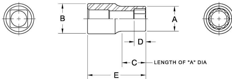
FIGURE 5 - TYPE I, CLASS I SOCKET STYLE A &amp; B
