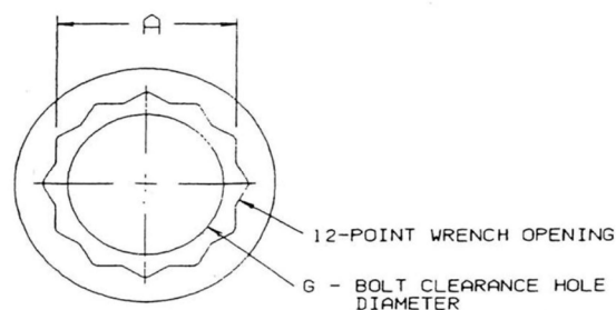
FIGURE 2B - BOLT CLEARANCE HOLE REQUIREMENT
