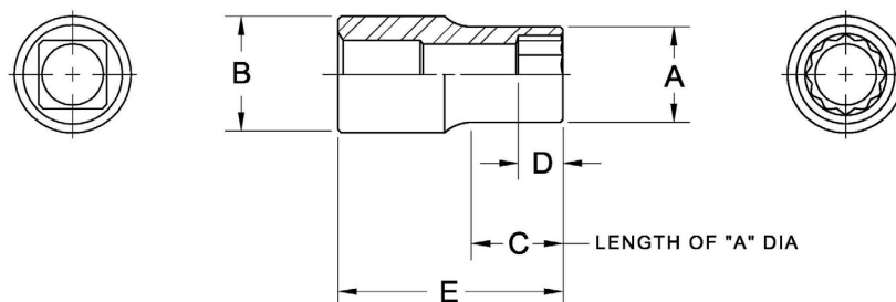
FIGURE 4 - TYPE I, CLASS I SOCKET STYLE A &amp; B
