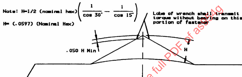
FIGURE 1A - INTERNAL WRENCH ENGAGEMENT
