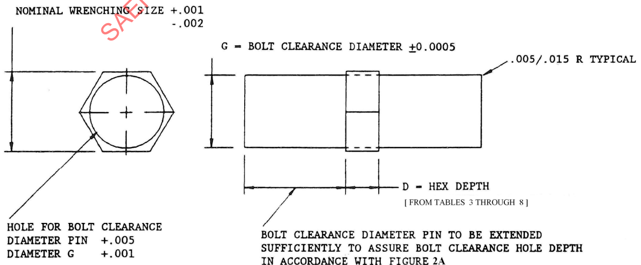
FIGURE 2C - BOLT CLEARANCE HOLE GAGE
