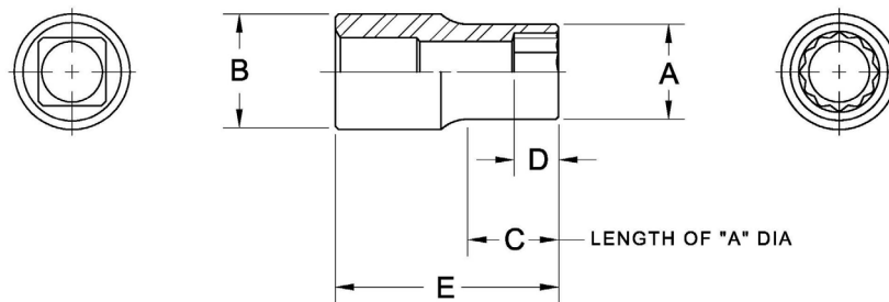
FIGURE 6 - TYPE I, CLASS I SOCKET STYLE A
