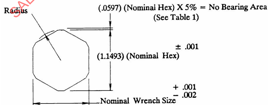
FIGURE 1B - MANDREL FOR WRENCH DESIGN TEST PROCEDURE
