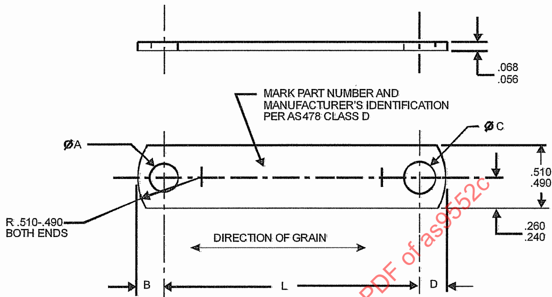
FIGURE 1 - BRACKET
