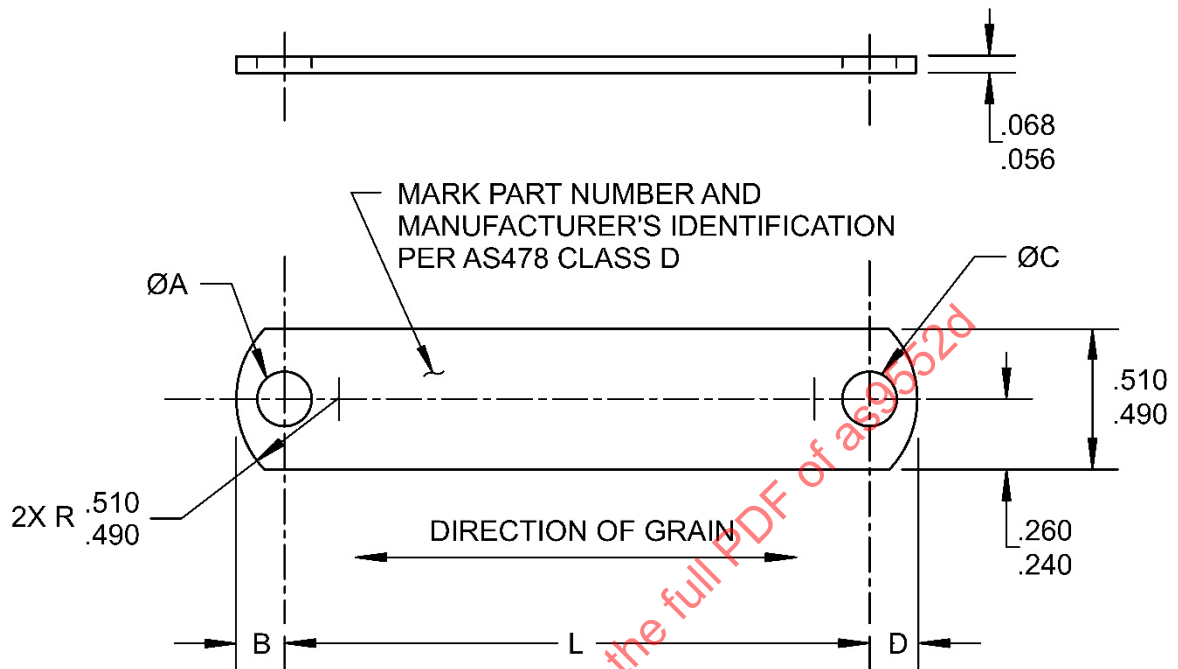
FIGURE 1 - BRACKET
