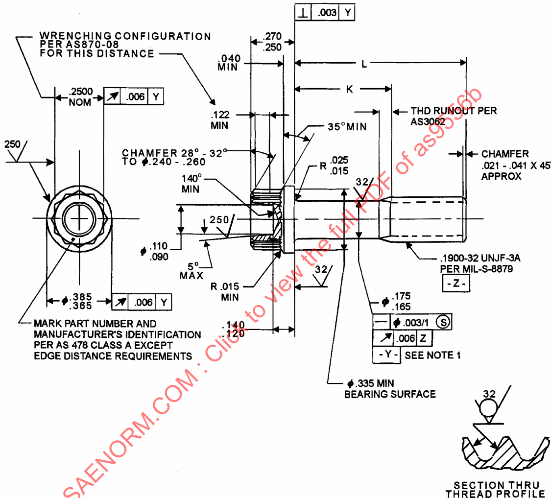
FIGURE 1 - BOLT
