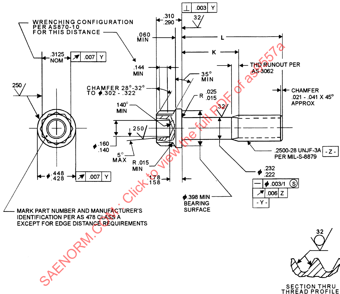
FIGURE 1 - BOLT
