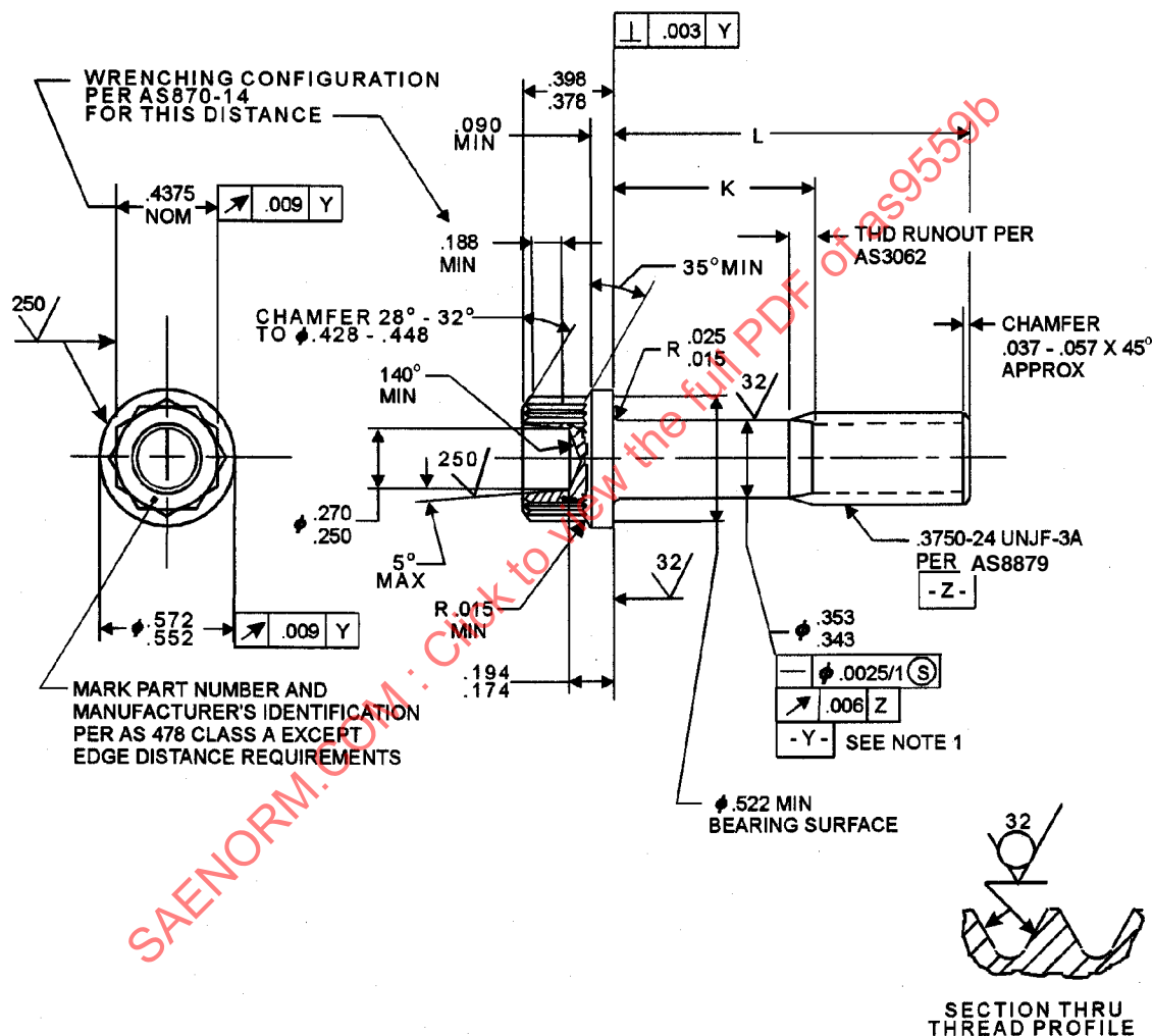
FIGURE 1 - BOLT
