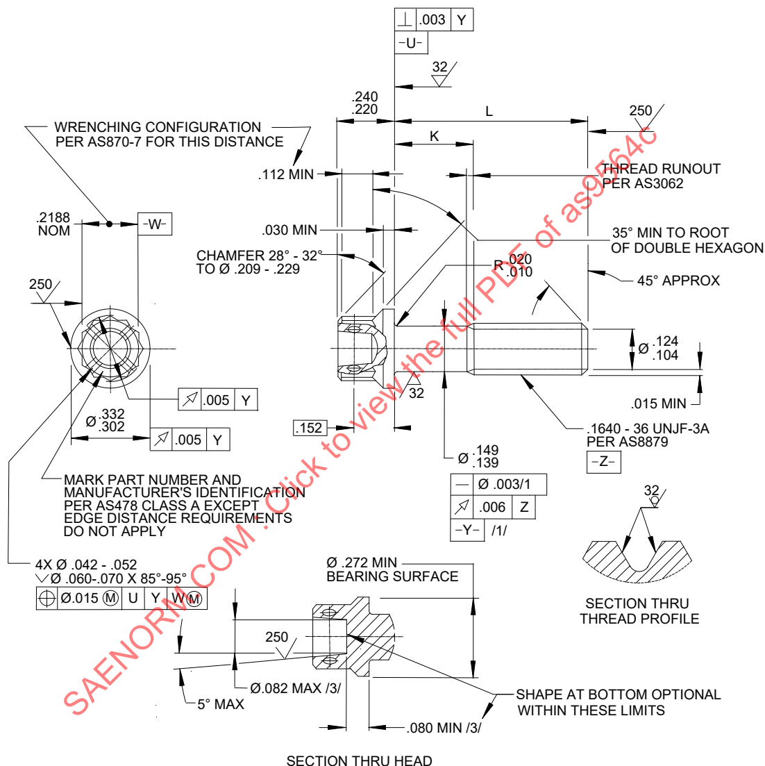
FIGURE 1 - SCREW
