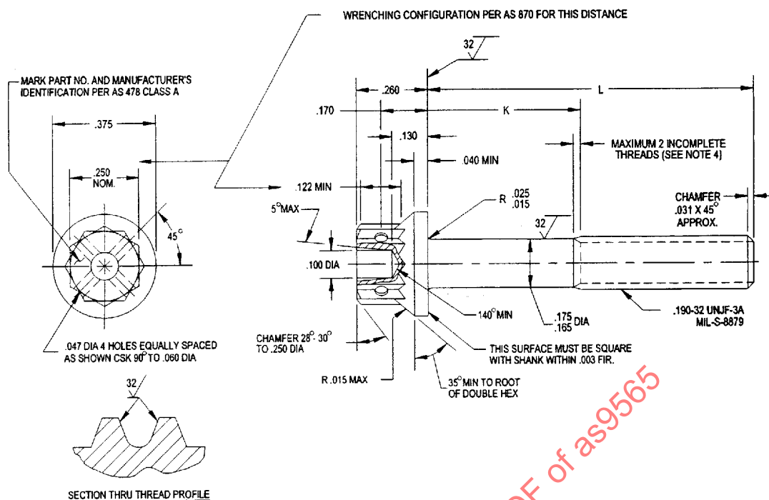
FIGURE 1 - BOLT
