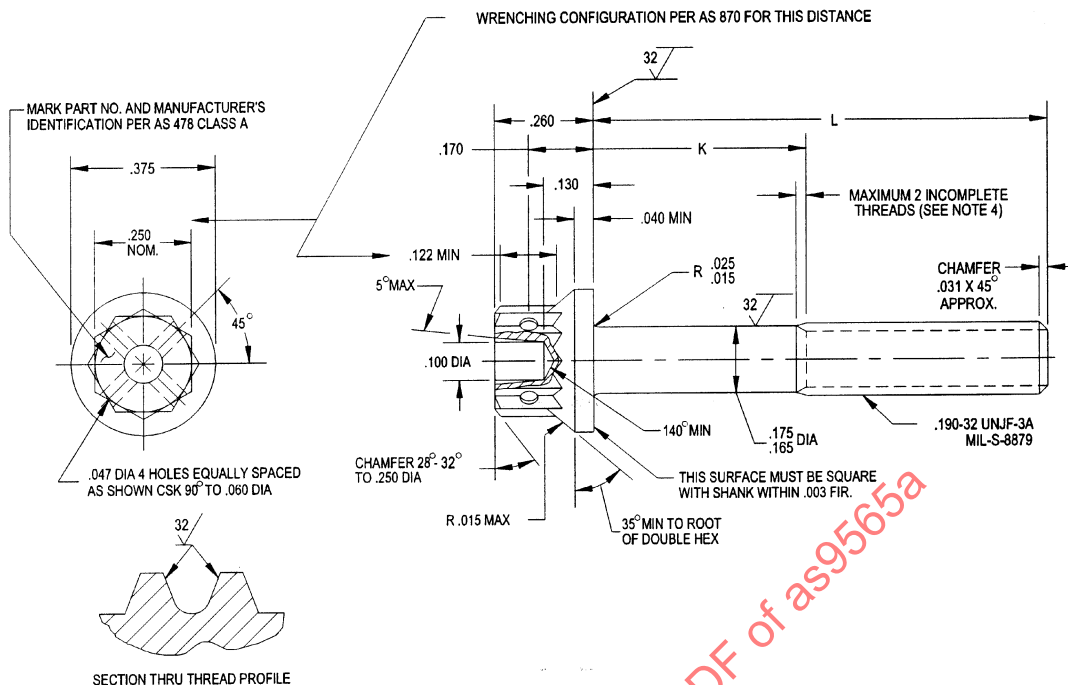
FIGURE 1 - BOLT
