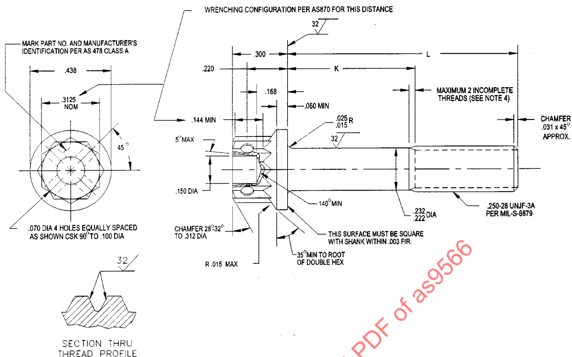
FIGURE 1 - BOLT
