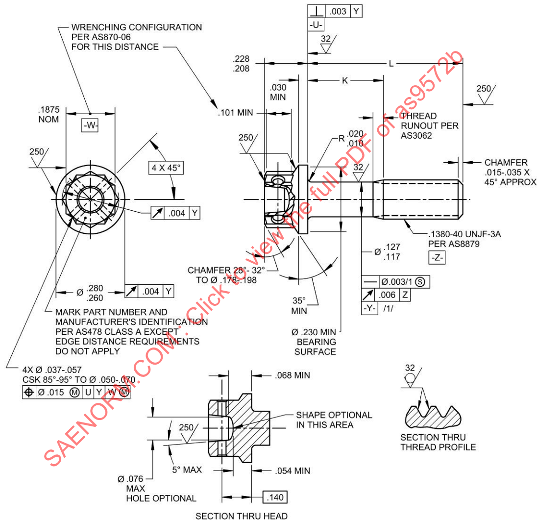
FIGURE 1 - SCREW
