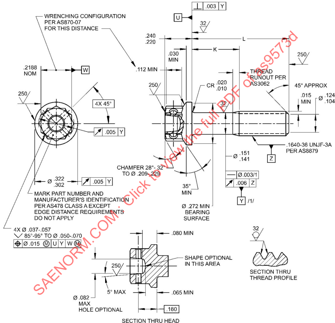
FIGURE 1 - SCREW
