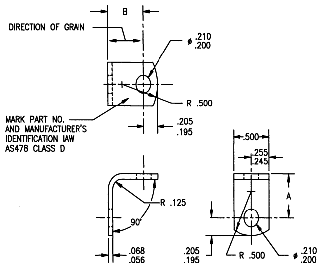
FIGURE 1 - ANGLE BRACKET
