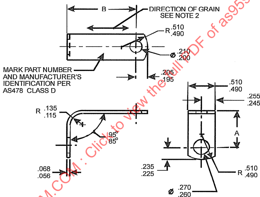
FIGURE 1 - ANGLE BRACKET
