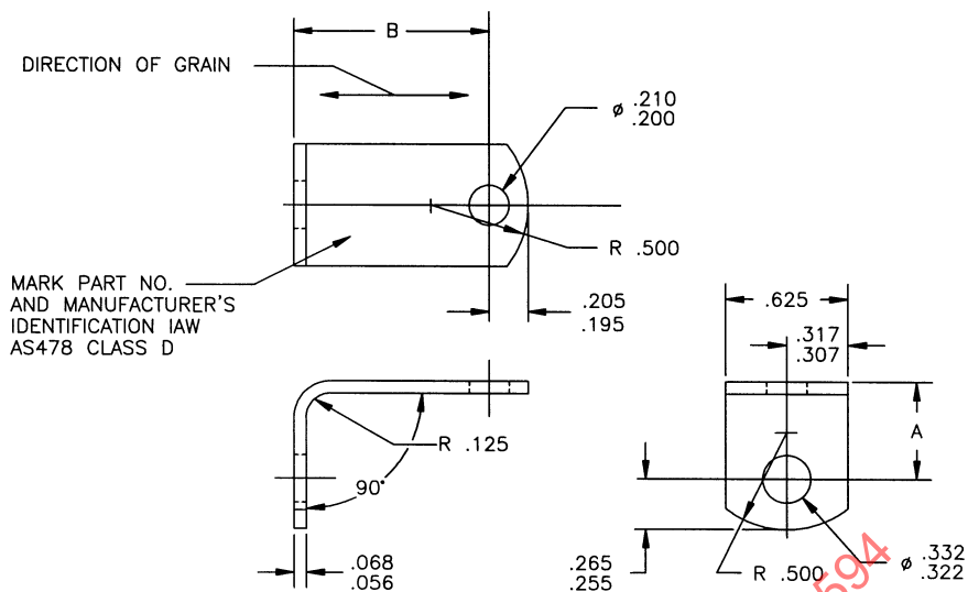
FIGURE 1 - ANGLE BRACKET
