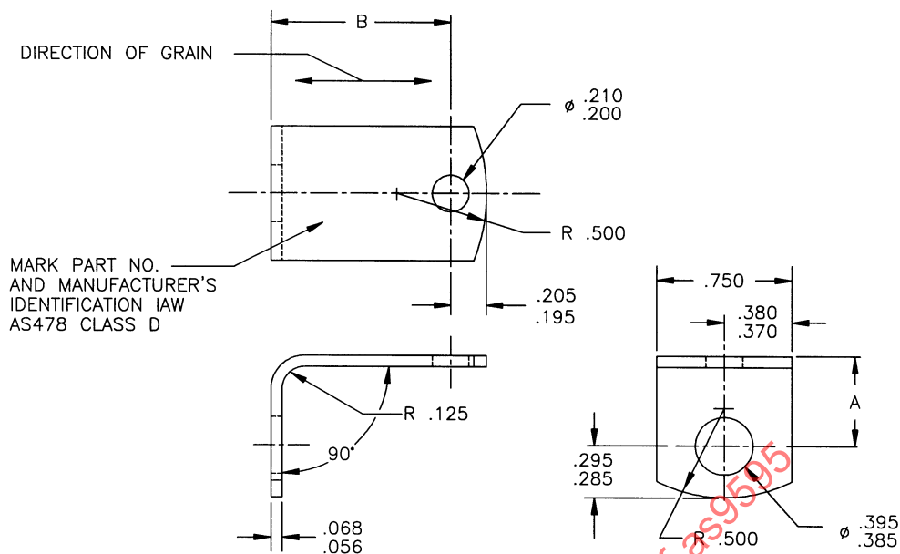
FIGURE 1 - ANGLE BRACKET
