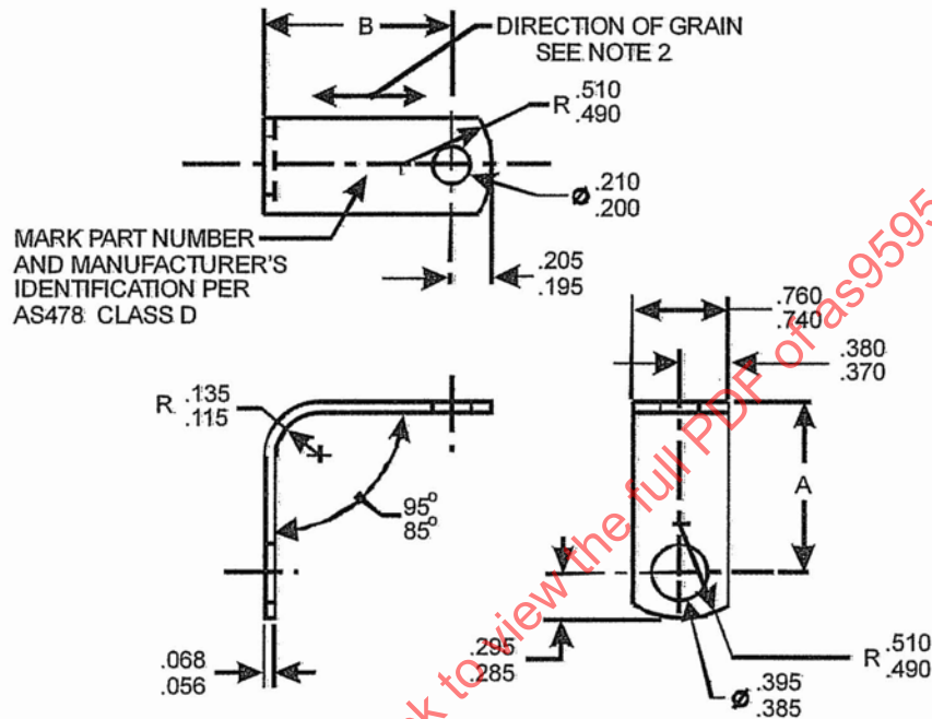
FIGURE 1 - ANGLE BRACKET
