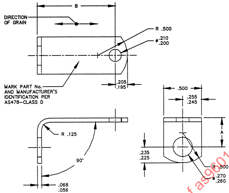
FIGURE 1 - ANGLE BRACKET
