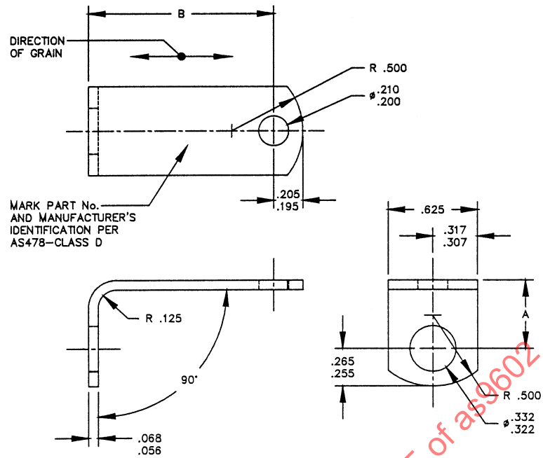
FIGURE 1 - ANGLE BRACKET
