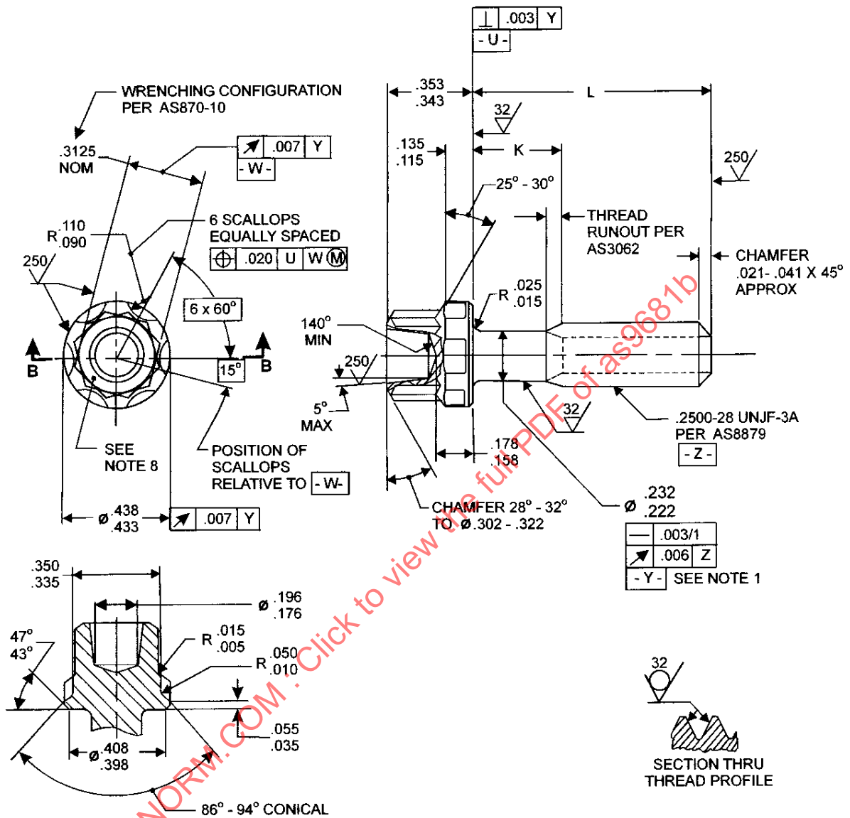
FIGURE 1 - BOLT
