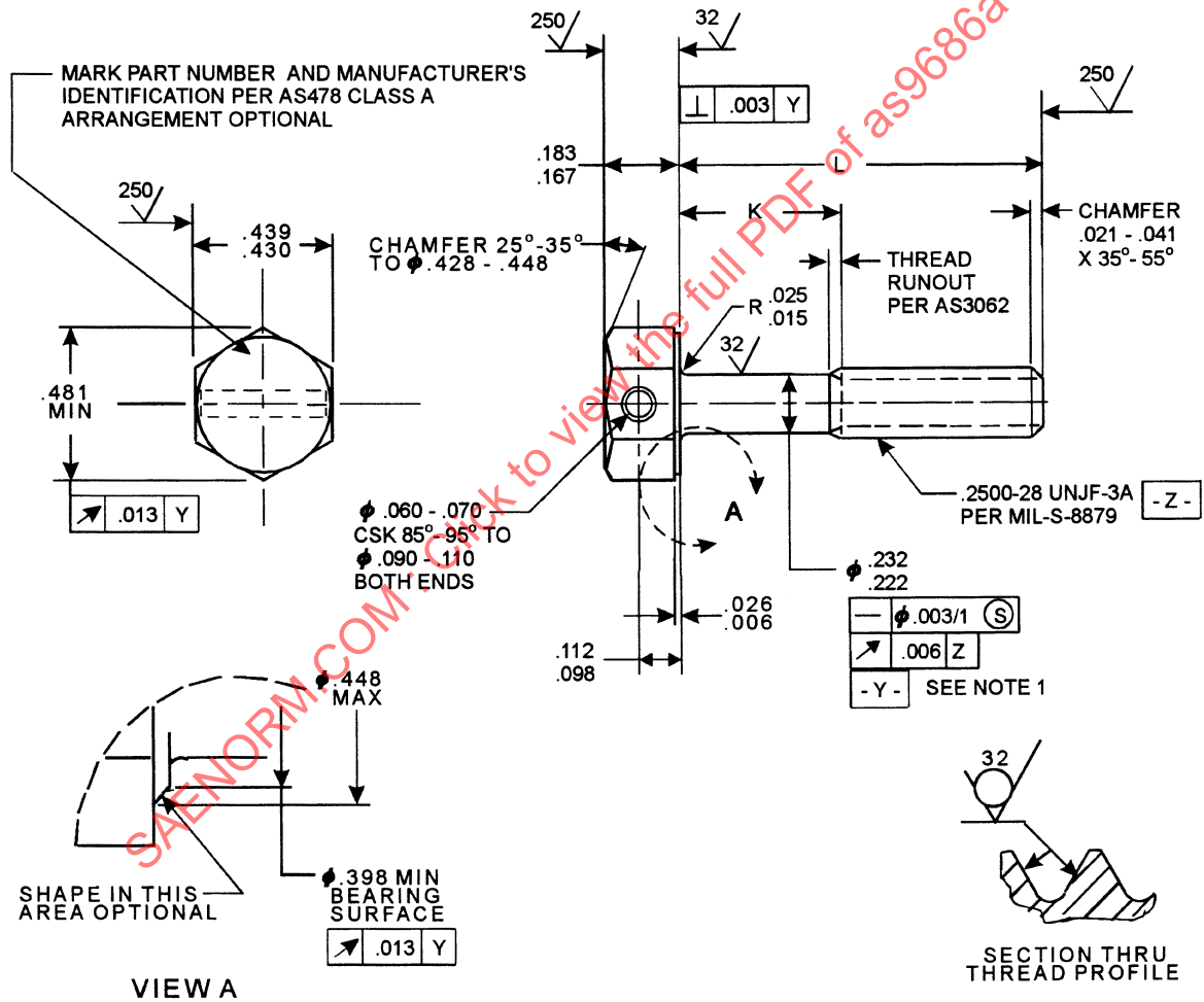
FIGURE 1 - BOLT
