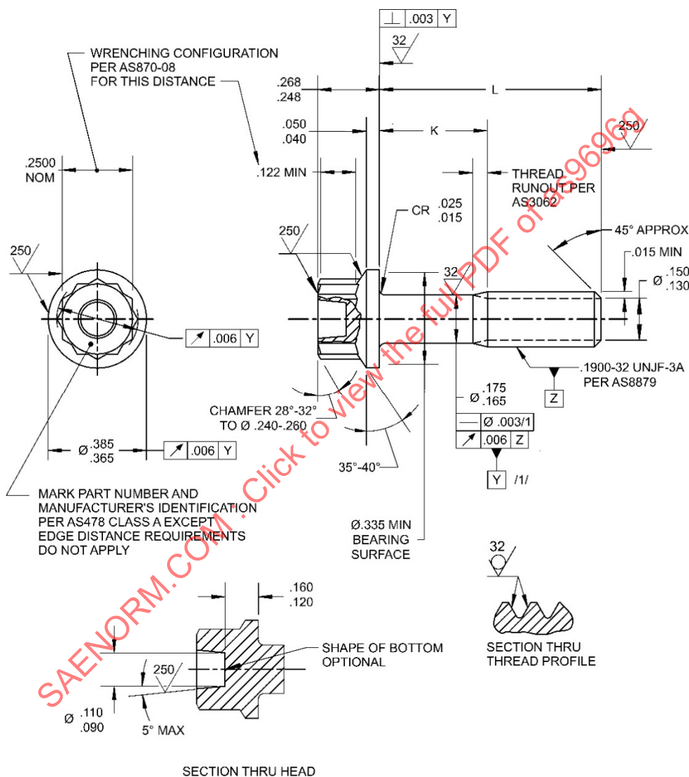
FIGURE 1 - BOLT
