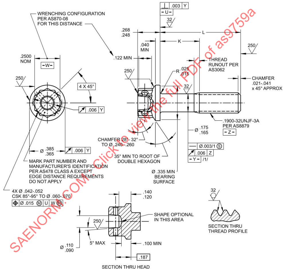
FIGURE 1 - BOLT
