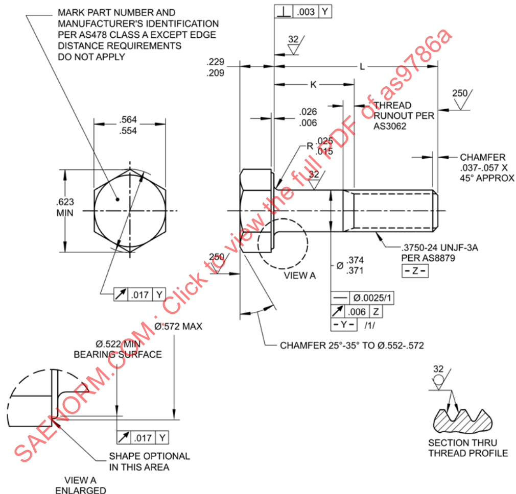
FIGURE 1 - BOLT
