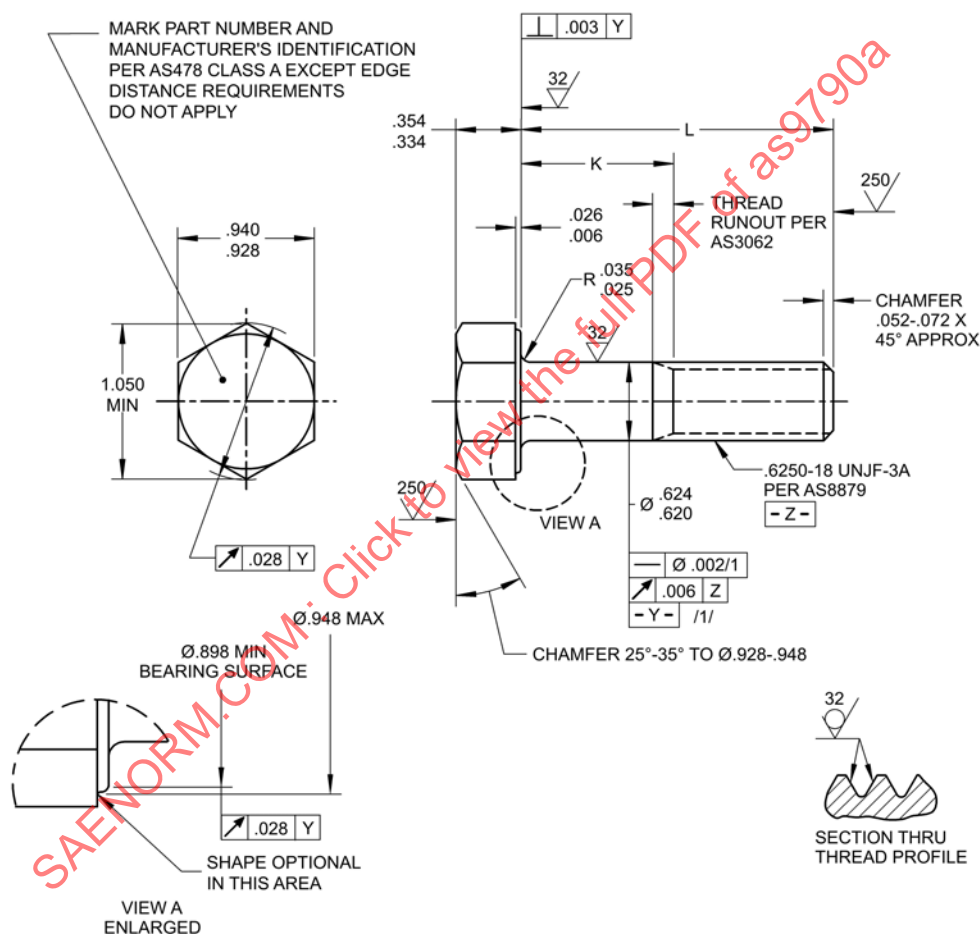
FIGURE 1 – BOLT
