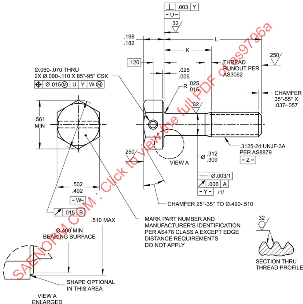
FIGURE 1 - BOLT
