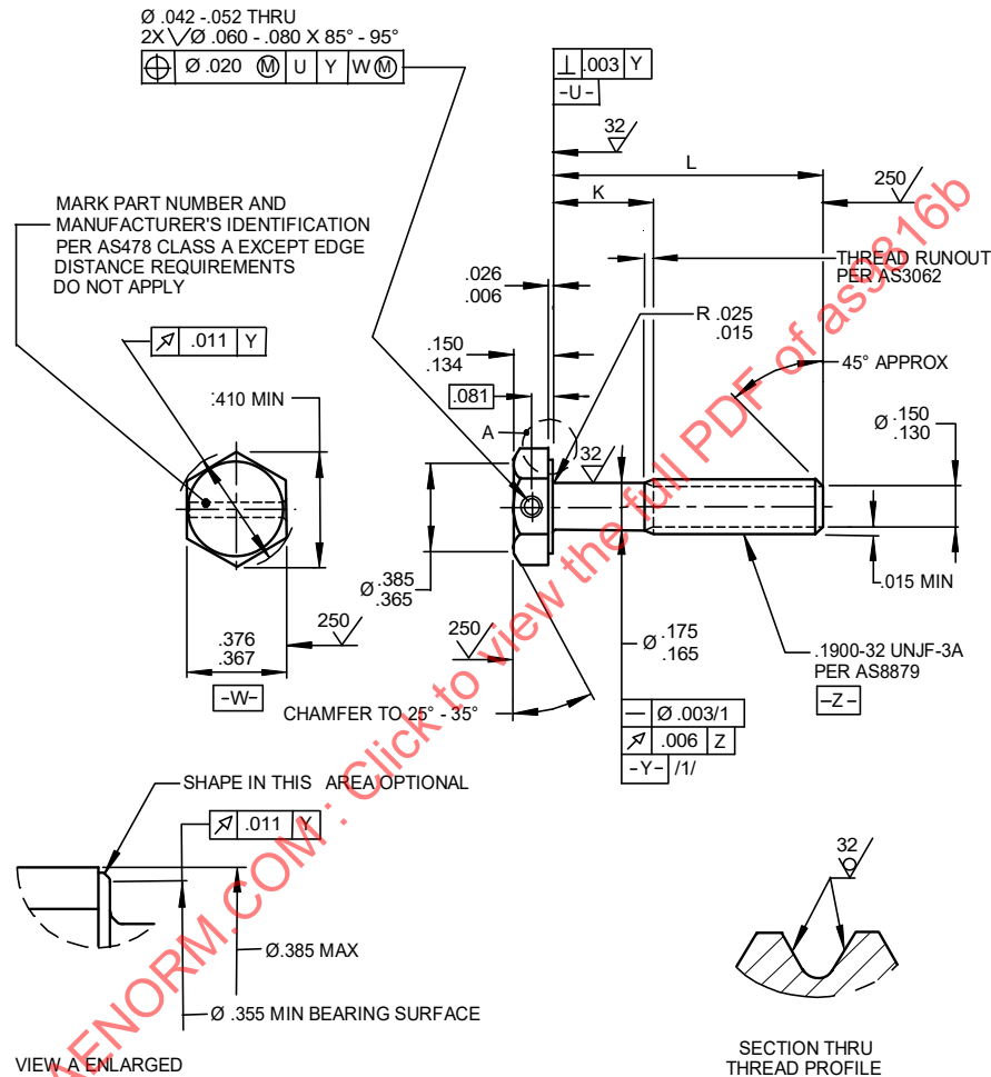
FIGURE 1 - BOLT
