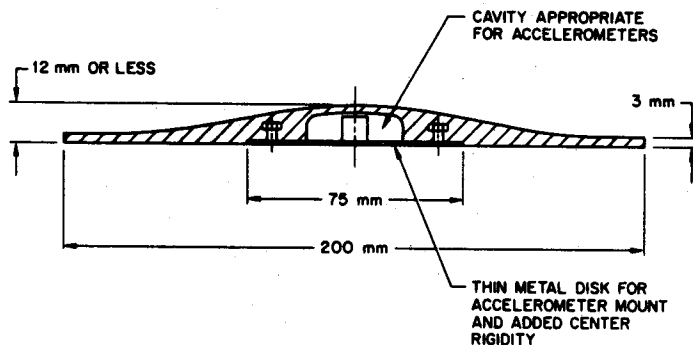
FIG. 3—SUGGESTED DESIGN FOR SEMI-RIGID DISC OF APPROXIMATELY 80-90 DUROMETER (A-SCALE) MOLDED RUBBER, PLASTIC, ETC.
