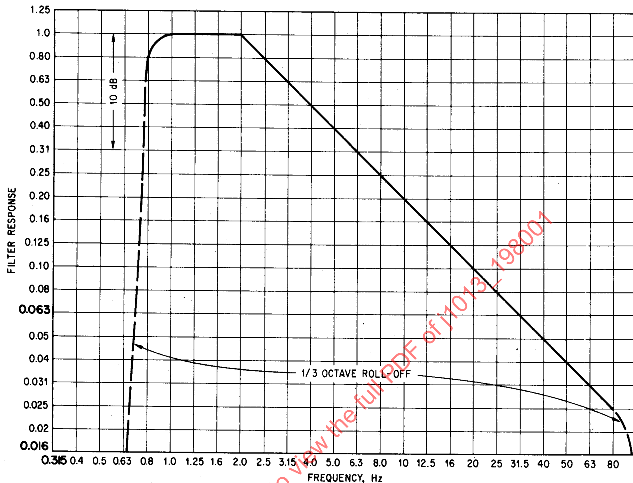
FIG. 5—FILTER RESPONSE FOR a_x and a_y
