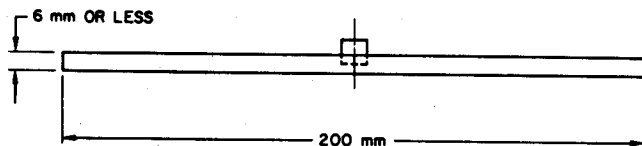
FIG. 2—SUGGESTED DESIGN FOR RIGID DISC WITH ACCELEROMETER ASSEMBLY BONDED AT CENTER
