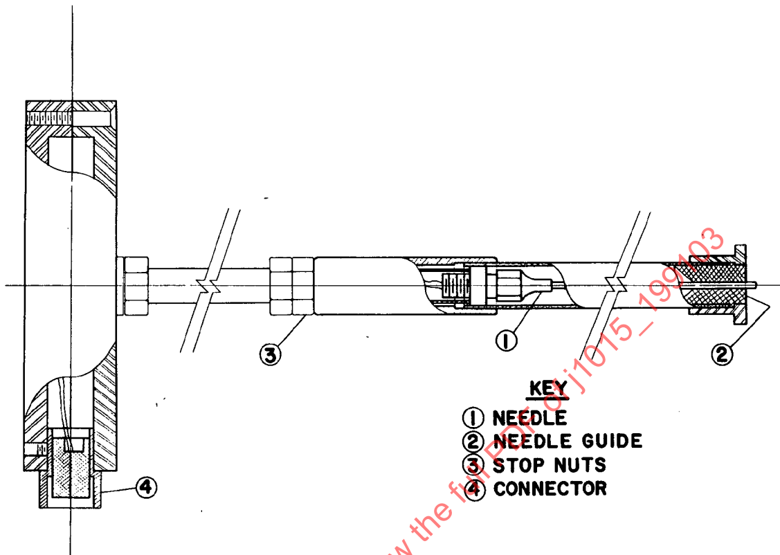
FIGURE 1 - Thermocouple Needle and Holder
