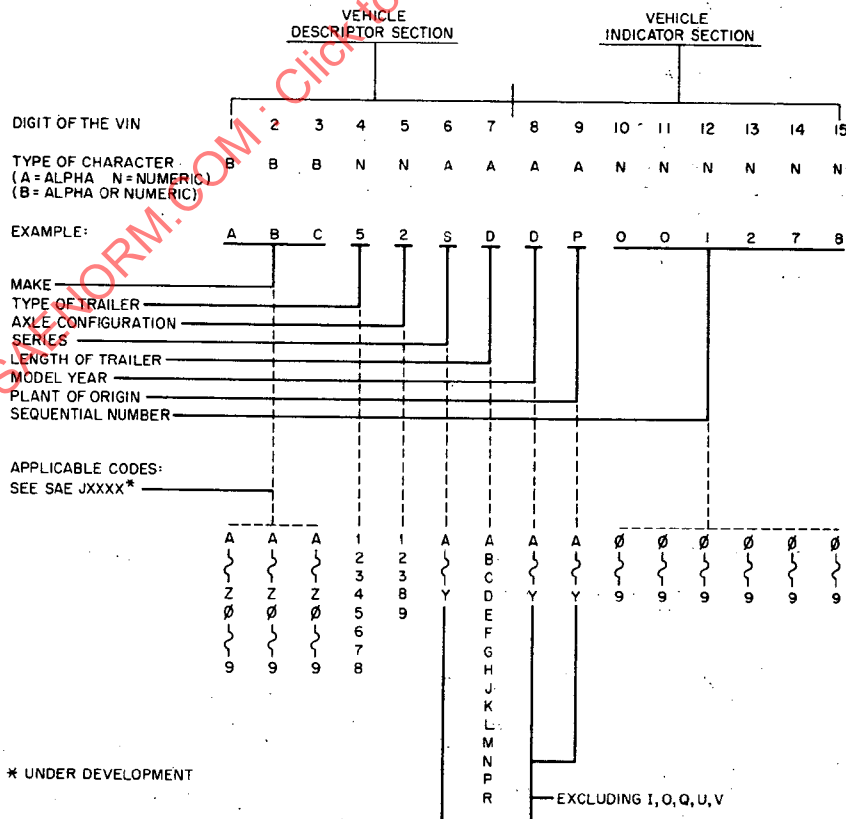
FIG. 1—RECREATIONAL TRAILER VEHICLE IDENTIFICATION NUMBER SYSTEM
