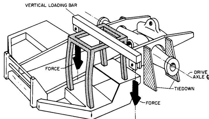
TYPICAL BUT NOT MANDATORY TEST CONFIGURATION
