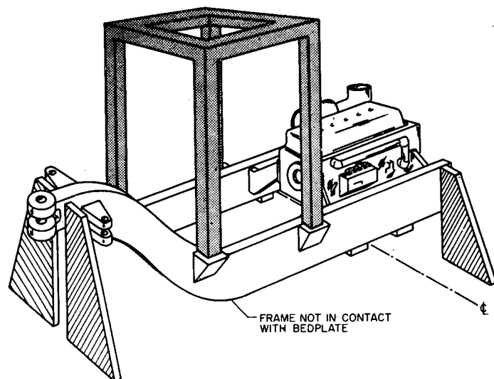
TYPICAL BUT NOT MANDATORY TEST CONFIGURATION
