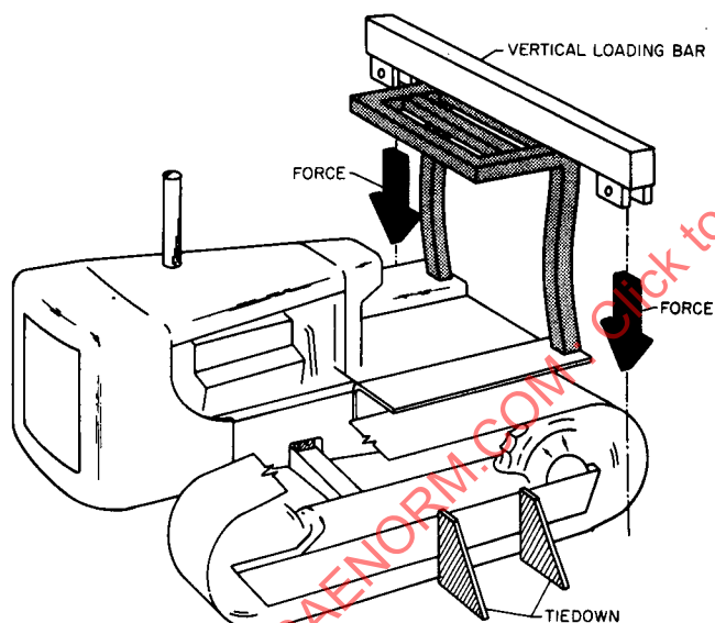
TYPICAL BUT NOT MANDATORY TEST CONFIGURATION
