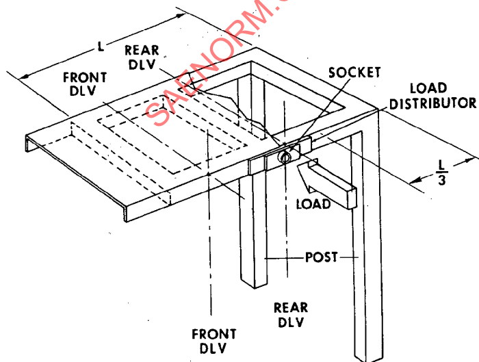
FIG. 1—LOAD DISTRIBUTOR AND SOCKET ARE TO PREVENT LOCAL PENETRATION AND TO HOLD END OF LOAD GENERATING DEVICE
