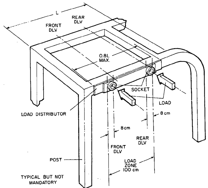
LOAD DISTRIBUTOR AND SOCKET ARE TO PREVENT LOCAL PENETRATION AND TO HOLD THE END OF LOAD GENERATING DEVICE
