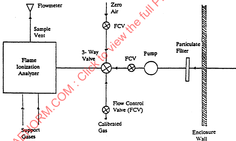
FIGURE 3—FID SAMPLE TRAIN
