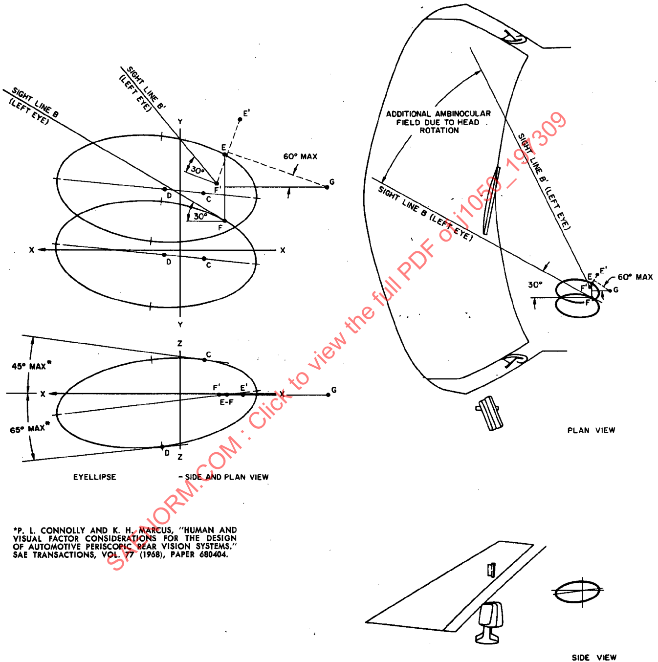
FIG. 5—AMBINOCULAR DIRECT FIELD OF VIEW WITH EYE AND HEAD MOVEMENT TO RIGHT
