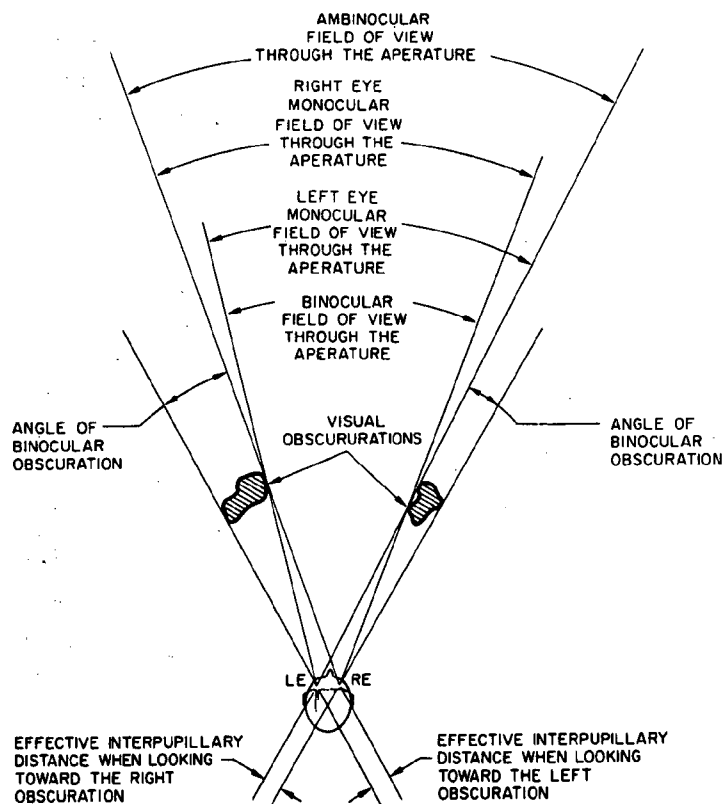
FIG. 2—DRIVER'S HORIZONTAL FIELD VIEW AS LIMITED BY OBSTRUCTIONS
