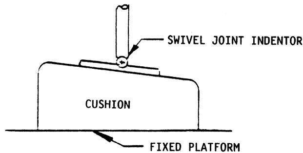
FIGURE 4—SWIVEL JOINT INDENTOR
