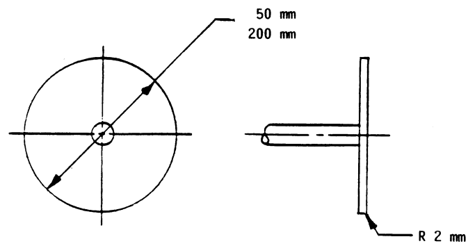
FIGURE 1—FLAT INDENTOR
