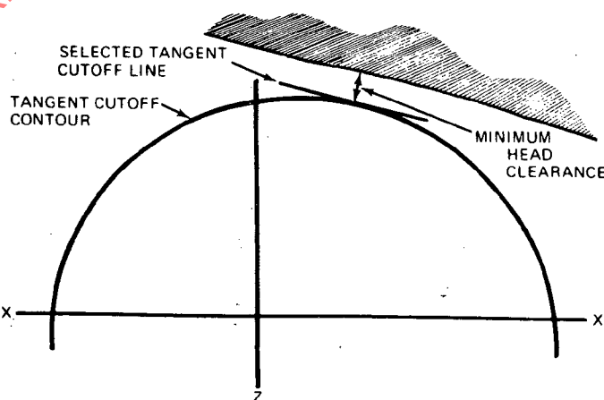
FIG. 1 - MINIMUM HEAD CLEARANCE
