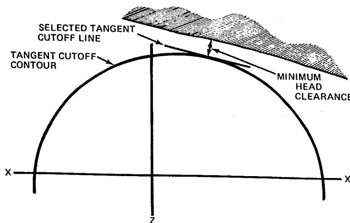
FIG. 1 - MINIMUM HEAD CLEARANCE
