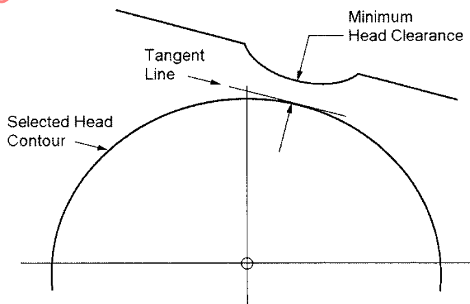
Figure 3 - Driver head position contours for Class A vehicles with seat track travel greater than 133 mm
