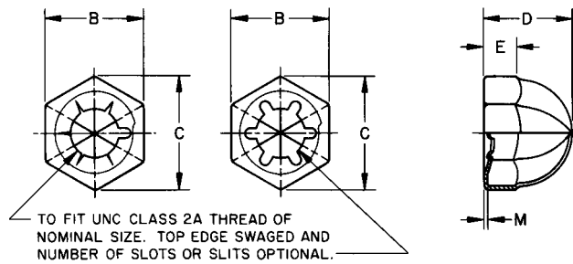
FIGURE 8—FORMED THREAD ACORN TYPE STAMPED NUTS
