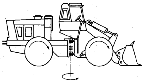
FIG. 3.2.2.1—FOUR WHEEL, ARTICULATED STEER, FOUR-WHEEL DRIVE, OPERATOR FRONT
