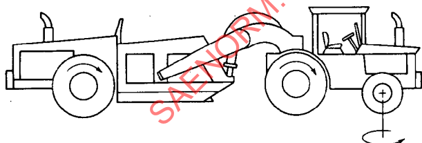
FIG. 5.1.5—THREE AXLES, FRONT-WHEEL STEER, CENTER- AND REAR-AXLE DRIVE
