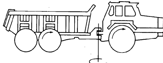
FIG. 4.1.2.3—THREE AXLES, FRONT- AND CENTER-AXLE DRIVE
