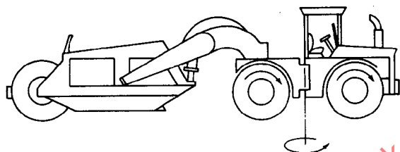
FIG. 5.1.3—THREE AXLES, ARTICULATED STEER, FRONT- AND CENTER-AXLE DRIVE (ARTICULATED TRACTOR OR FOUR-WHEEL STEER TRACTOR)
