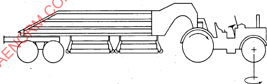
FIG. 4.3.1.3—FOUR AXLES, SINGLE-AXLE DRIVE, TANDEM TRAILING AXLES
