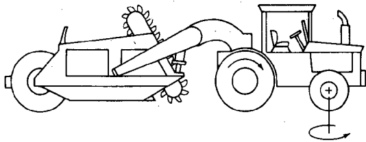
FIG. 5.2.3—THREE AXLES, FRONT-WHEEL STEER, CENTER-AXLE DRIVE
