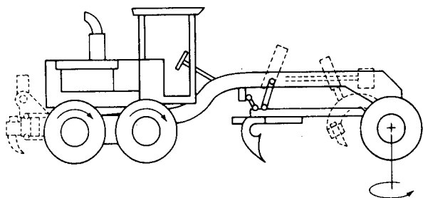
6.1.3 SIX WHEEL, FRONT WHEEL STEER, FOUR WHEEL DRIVE
