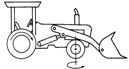
3.2.1.1 FOUR WHEEL, FRONT-WHEEL STEER, REAR-WHEEL DRIVE, FRONT ENGINE
