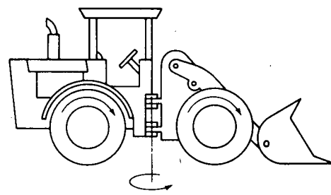
3.2.2.2 - FOUR WHEEL, ARTICULATED STEER, FOUR-WHEEL DRIVE, OPERATOR REAR
