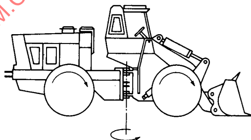
3.2.2.1 - FOUR WHEEL, ARTICULATED STEER, FOUR-WHEEL DRIVE, OPERATOR FRONT
