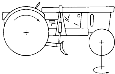
6.1.1 FOUR WHEEL, FRONT WHEEL STEER, TWO WHEEL DRIVE (FRONT ENGINE)
