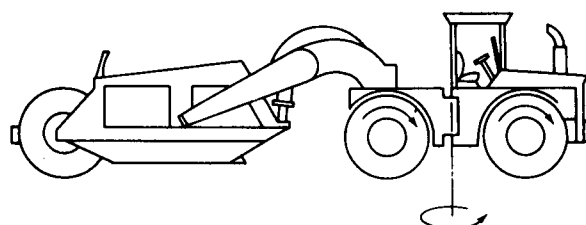
5.1.3 THREE AXLES, ARTICULATED STEER, FRONT AND CENTER AXLE DRIVE (ARTICULATED TRACTOR OR FOUR-WHEEL STEER TRACTOR)
