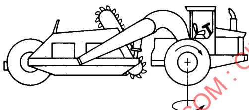
5.2.1 TWO AXLES, ARTICULATED STEER, FRONT AXLE DRIVE
