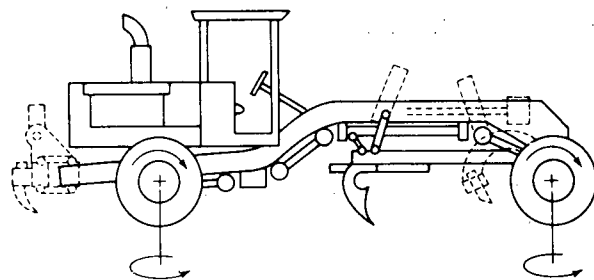
6.1.2 FOUR WHEEL, FRONT AND REAR WHEEL STEER, FOUR WHEEL DRIVE
